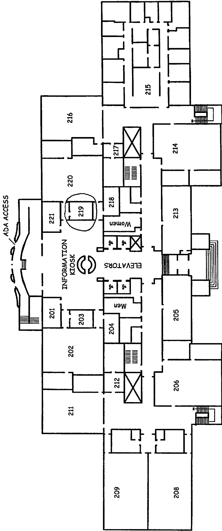
SECOND FLOOR PLAN BURTON CROSS BUILDING
